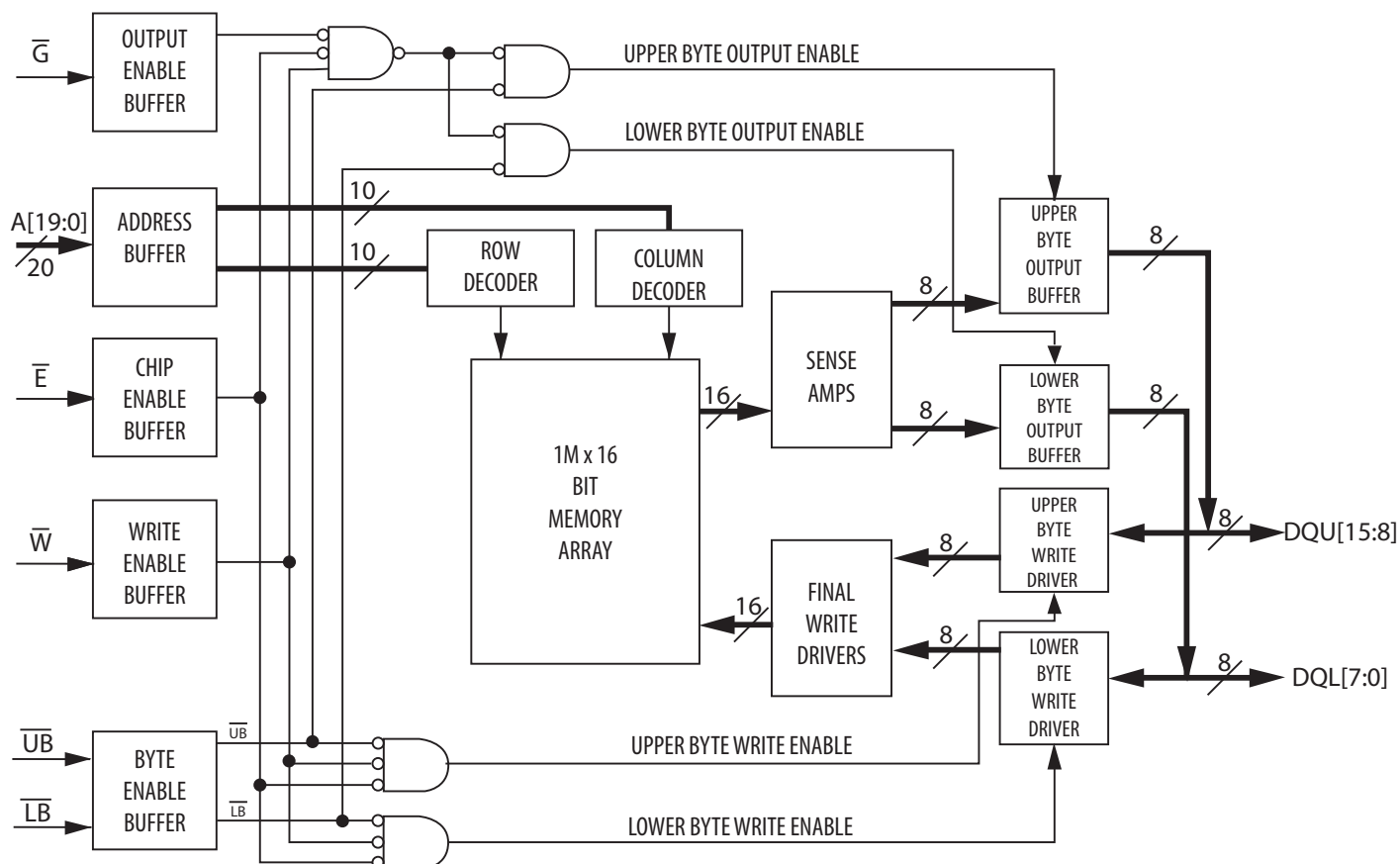
Figure 1.1 Block Diagram
